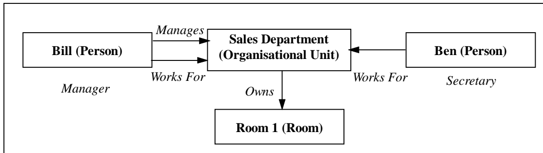
Figure 4: Example Organisational Model
