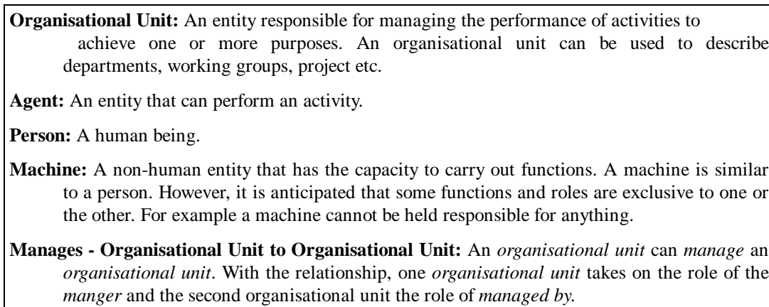
Figure 2: Definition of the Concepts in the Organisational Modelling Language
