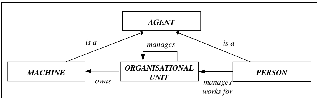
Figure 3: Graphical Representation of the Organisational Structure Modelling Language
