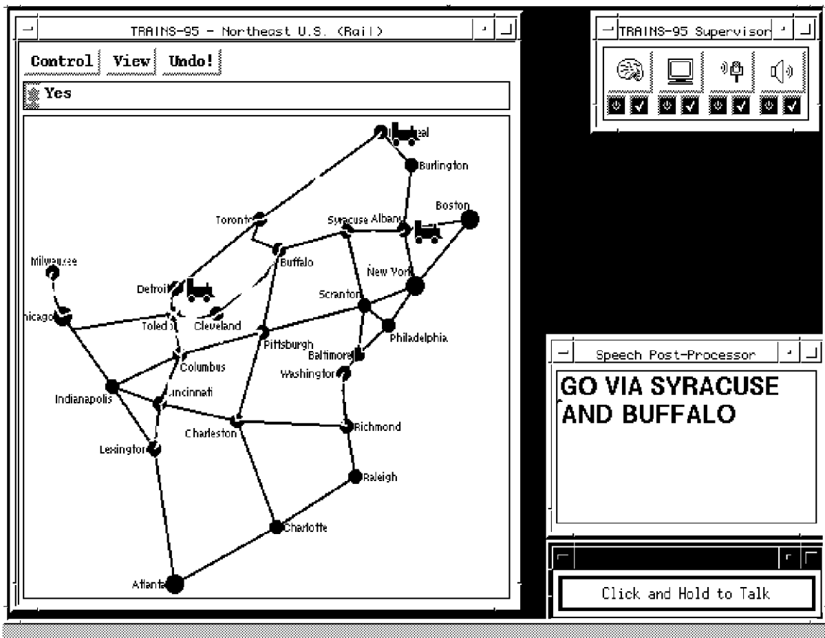
Figure 7: TRAINS Interface
