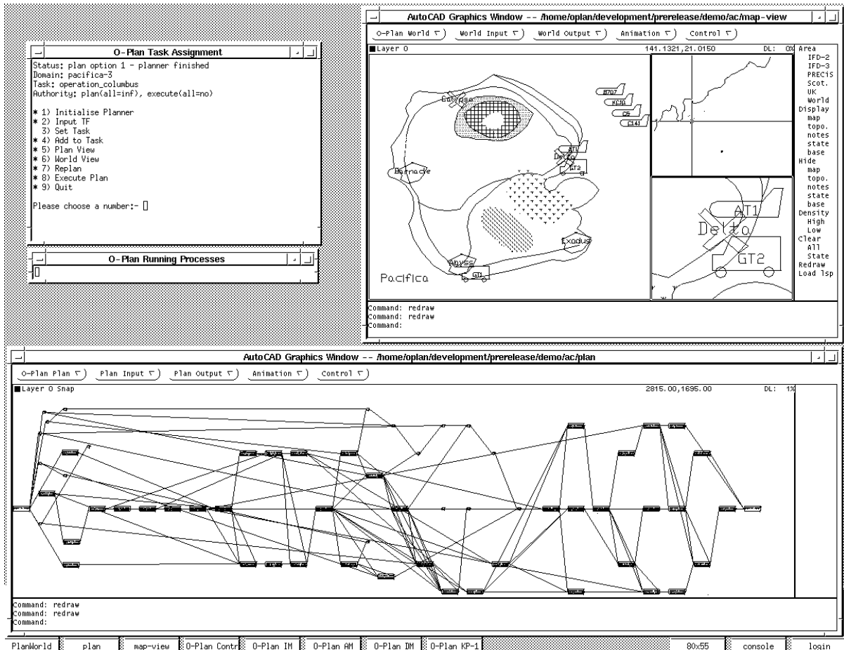
Figure 6: O-Plan PlanWorld Viewer User Interface
