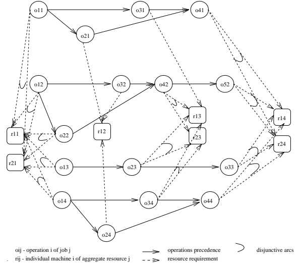
Figure 2: The representation of the job shop scheduling problem
