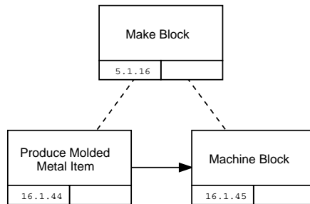
Figure 27: Process for manufacturing the 350-Block
