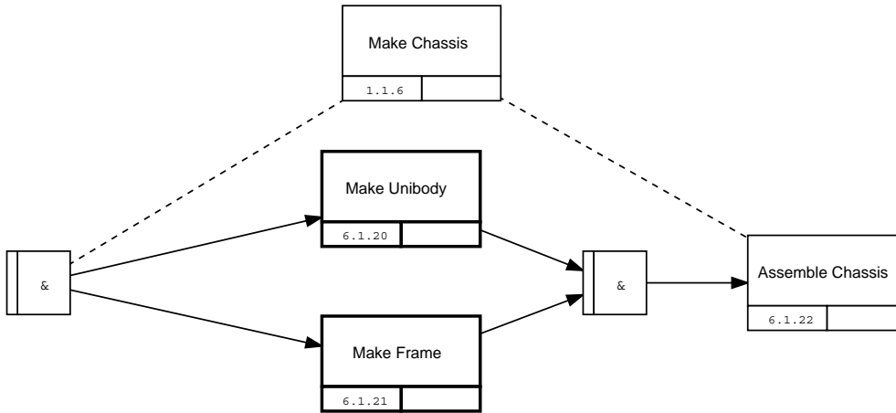
Figure 31: Process for manufacturing the 350-Chassis
