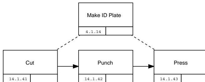
Figure 25: Process for manufacturing the 350-ID Plate
