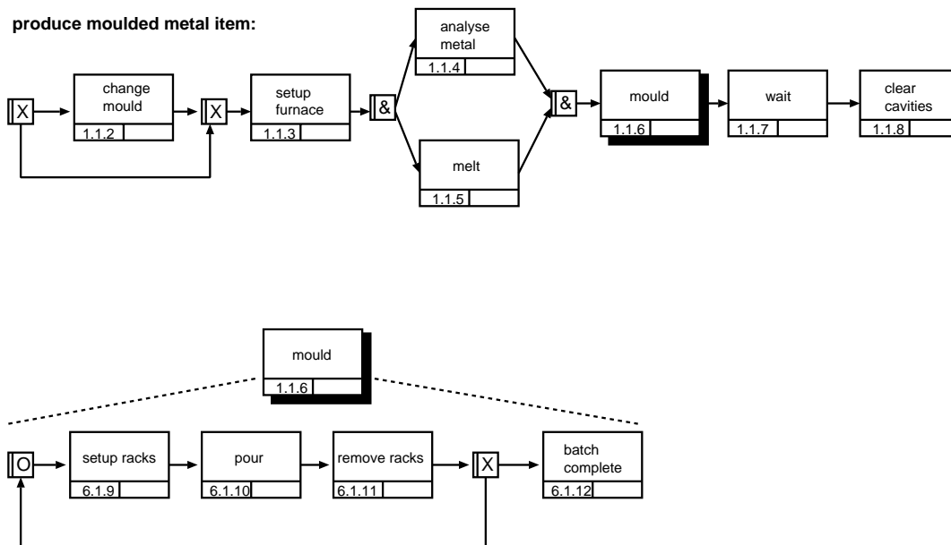
Figure 1: Production steps in the foundry
