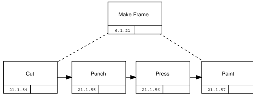
Figure 33: Process for manufacturing the 350-Frame
