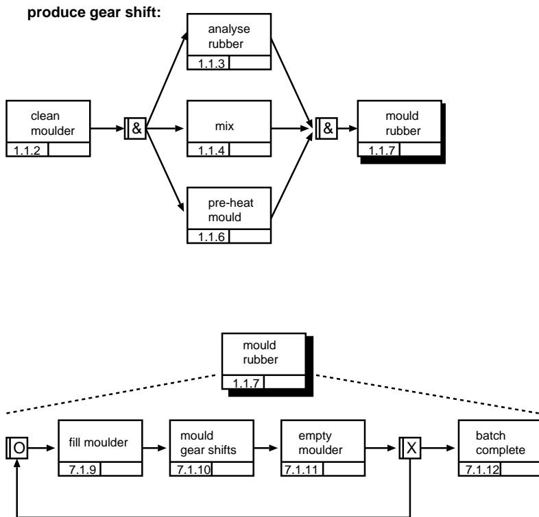
Figure 4: Production steps in the rubber works
