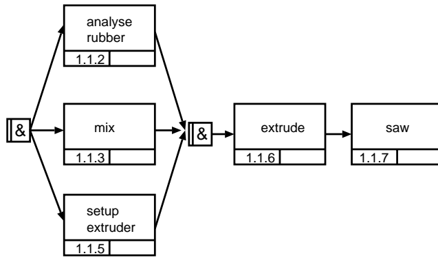
Figure 3: Production steps in the rubber works
