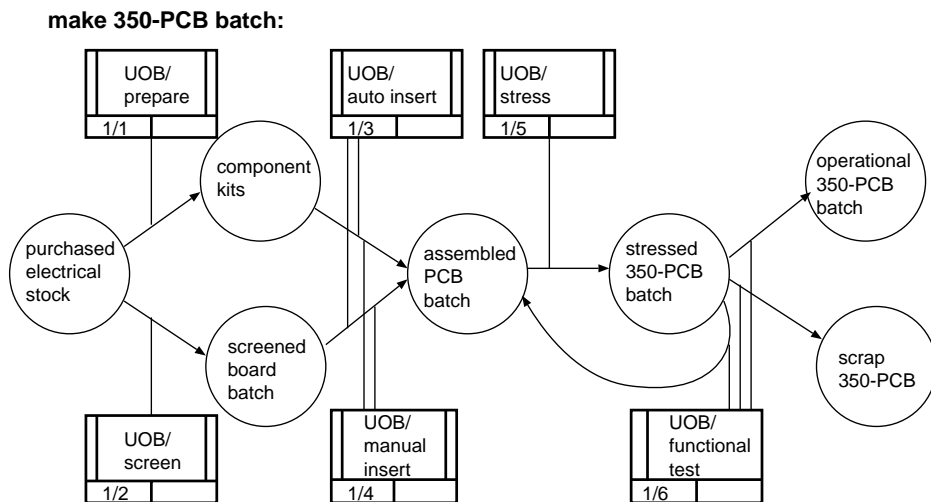
Figure 14: Object state transitions in the Electronics department
