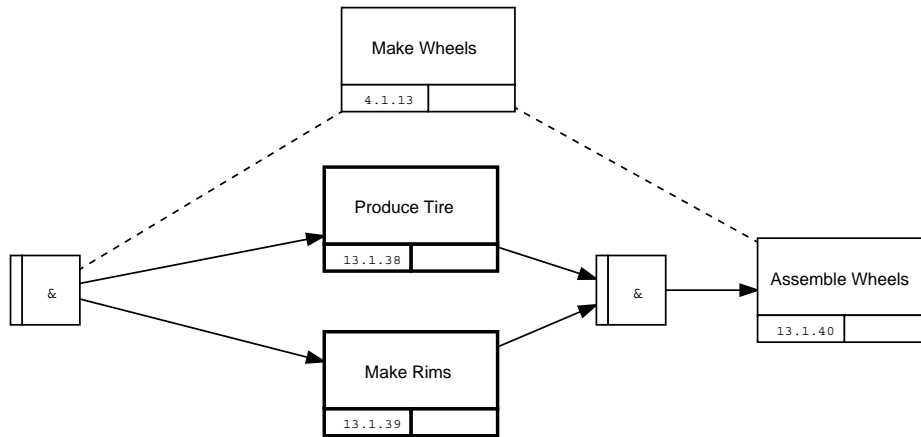
Figure 24: Process for manufacturing the 350-Wheels
