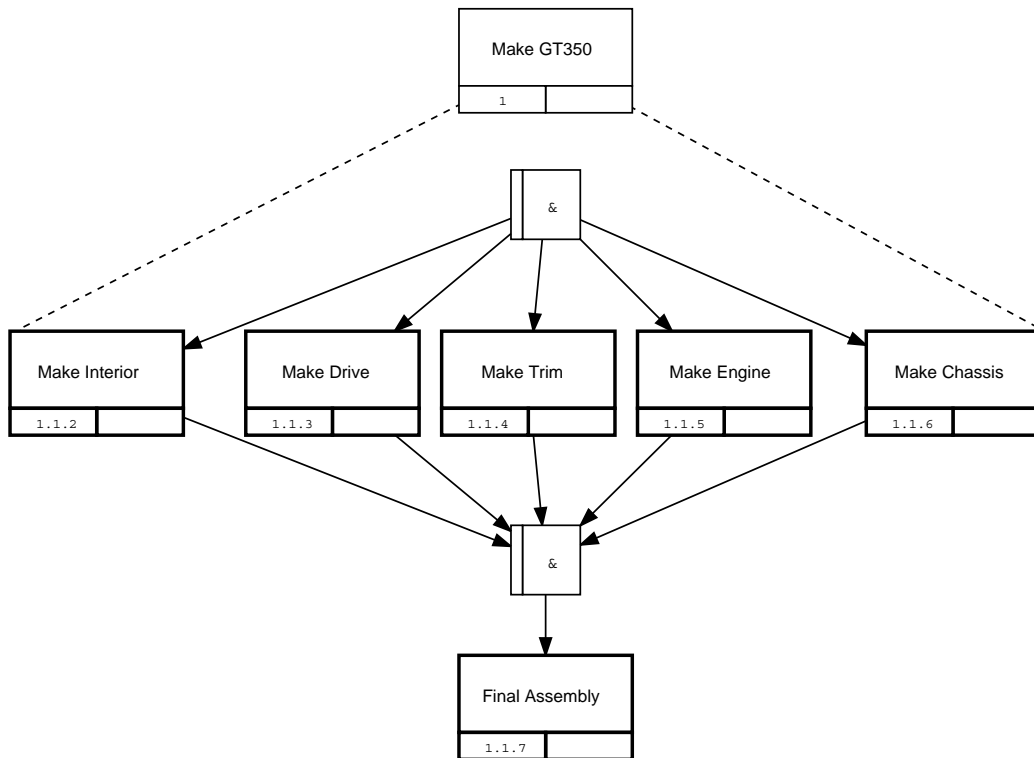
Figure 19: Top level process for manufacturing a GT-350
