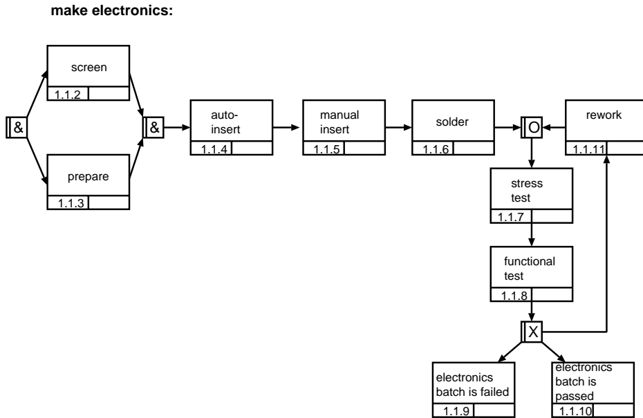
Figure 13: Production steps in the Electronics department
