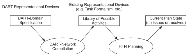
Figure 11: DART-Network Architecture
