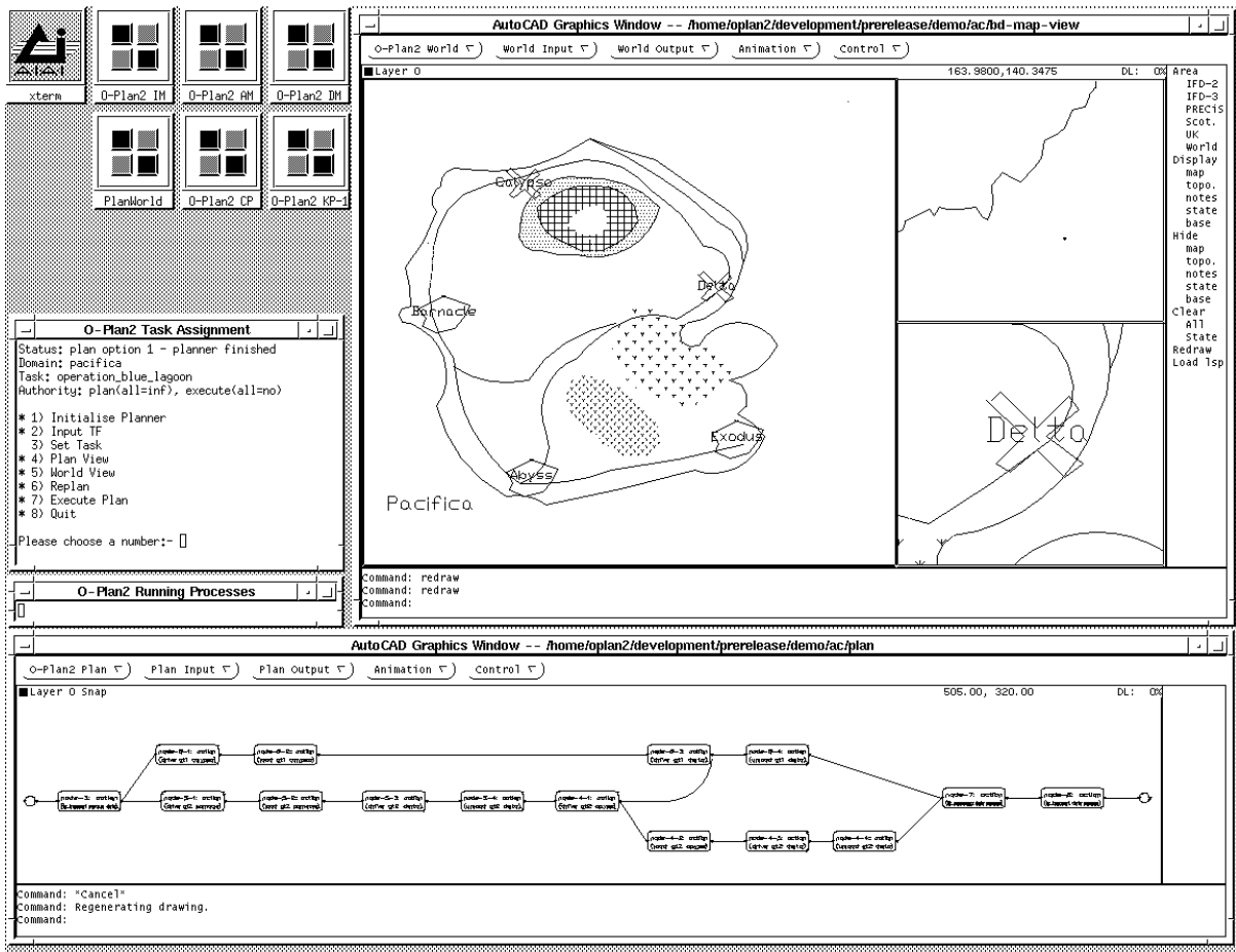
Figure 3: PlanWorld User Interface for Non-Combatant Evacuation Operations
